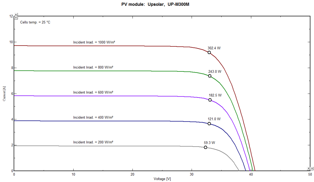
I-V curve of UP-M300M for different irradiance levels
