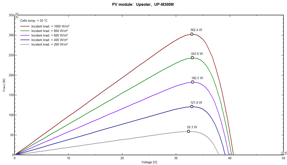
P-V curve of UP-M300M for different irradiance levels
